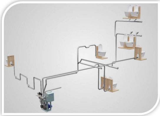
VacDrain Vacuum Toilet System
