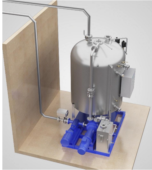
2 pumps solution 1 vacuum pump 1 discharge pump Tank volume can be customized
